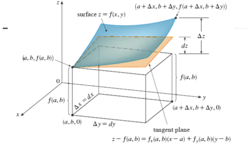
Figure 1.2.1: Geometrical interpretation of the differential (two variables)
