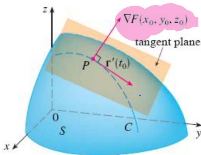
Figure 6.0.1: Tangent planes to level surfaces
